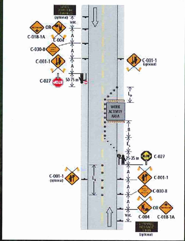
Figure 7.0: Lane Closure with TCPs – Single Lane Alternating – Short and Long Dur
